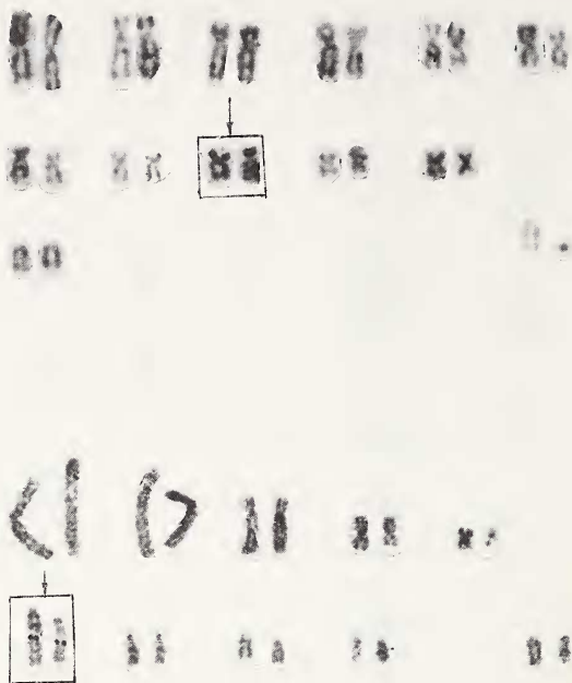
Fig. 2: NOR-banding. Karyotypes of a) S. subtilis nordmanni , male from Donetsk district, Chotumovski steppe ( 2n = 26 , NF = 48 ); b) S. severtzovi , female from Kursk region, Central Chernozem Reserve ( 2n = 20 , NF = 30 ).
